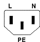
IEC 320 / C13
