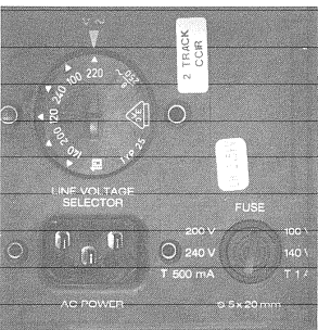
Mains connector
